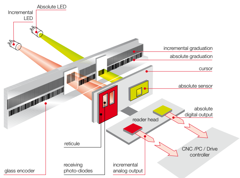
Graduated glass encoder
